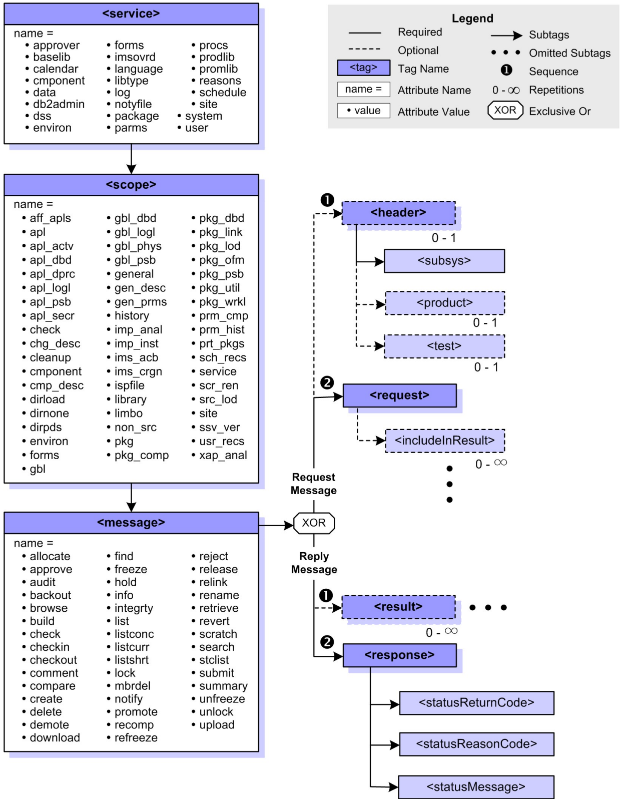
Exhibit 3-3. High-Level XML Document Structure
