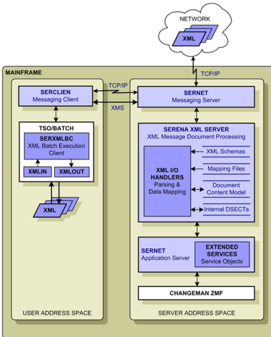
Exhibit 2-1. XML Services Architecture
